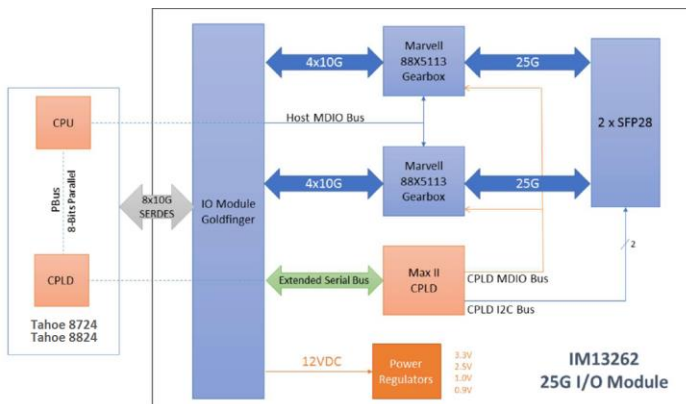
Block Diagram of IM13262 (I/O module with 2 ports of 25G SFP28)
