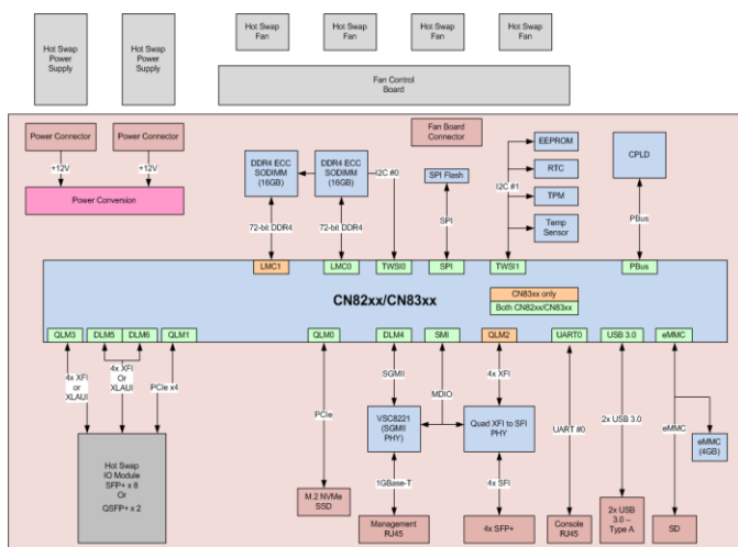
Block Diagram of Tahoe 8824
