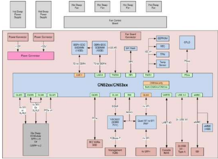
Block Diagram of Tahoe 8824
