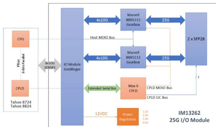
Block Diagram of IM13262 (I/O module with 2 ports of 10/25G SFP28)
