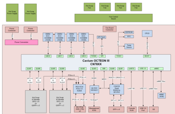
Block Diagram of Tahoe 8724
