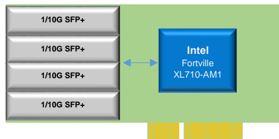
Block Diagram of Sierra 3121
