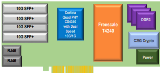
Block Diagram of Sierra 732
