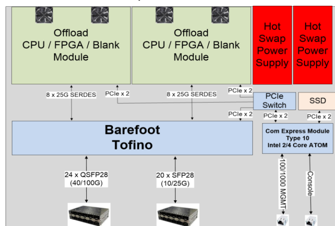
Block Diagram of Tahoe 2624
