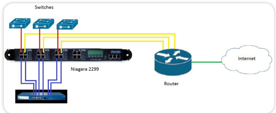
Palo Alto Networks next-generation firewall with Interface Masters Niagara bypass switch
