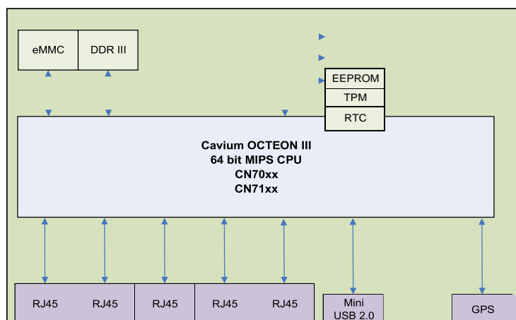
Block Diagram of Tahoe 8718
