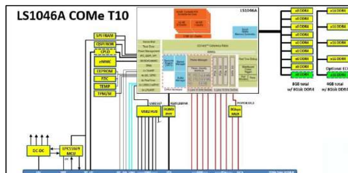
Block Diagram showing the COM Express Type 10 with LS1046A
